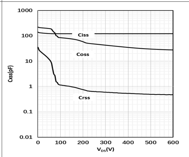
Figure 19 Typ. capacitances
