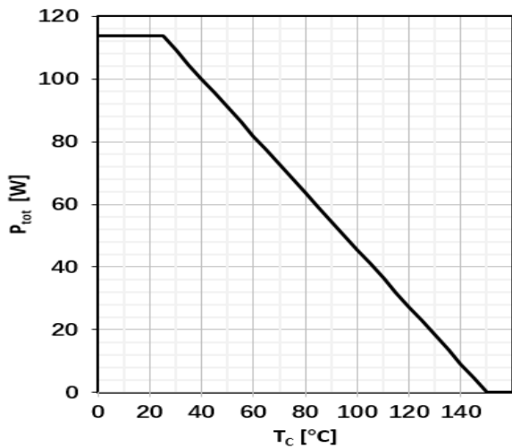
Figure 14 Power dissipation
